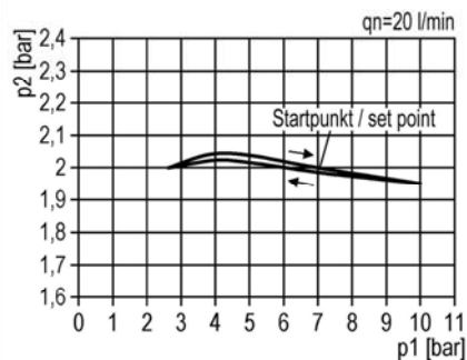
pressure characteristic
