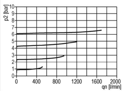
exhaust characteristics
